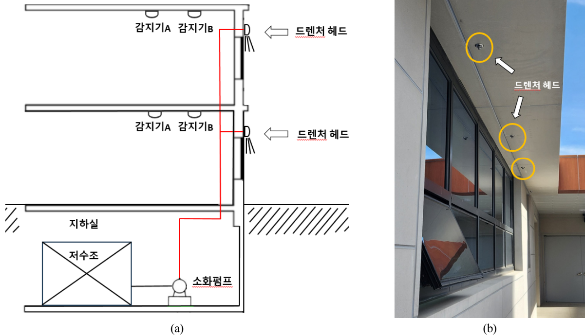
Fig. 1. (a) Schematic drawing of drencher facility (b) Picture image of installation of drencher facility
